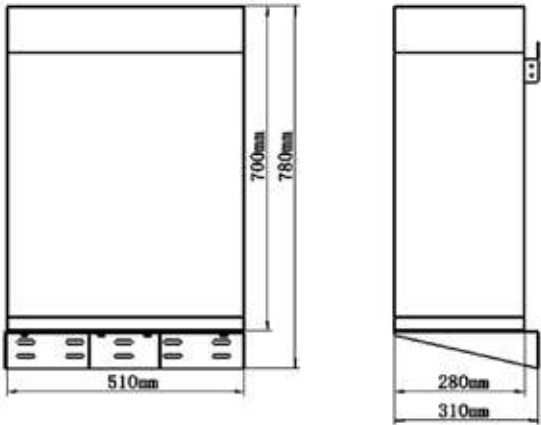
Mechanical drawing
